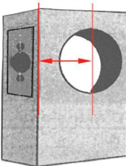
Backset (usually 2-3/8" or 2-3/4")
